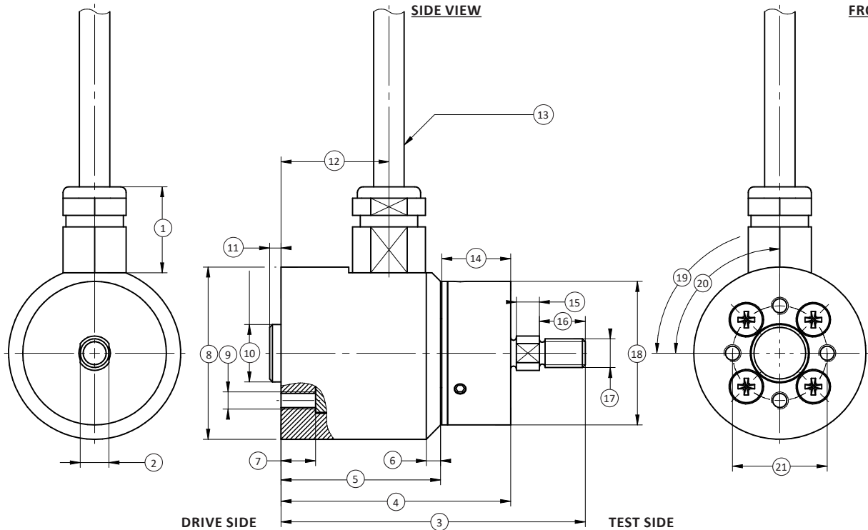
SIDE VIEW
